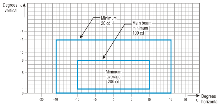
Figure A2-12. Isocandela diagram for taxiway centre line (15 m spacing)
